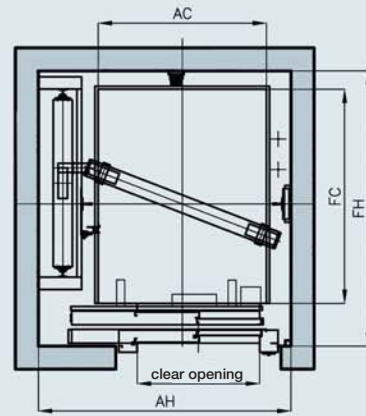
Plan view of shaft
