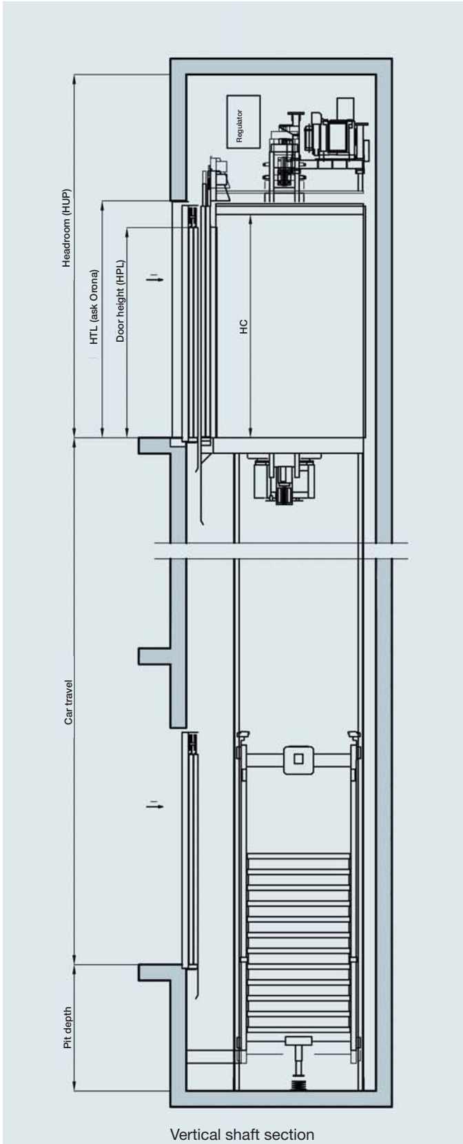
Shaft side view
